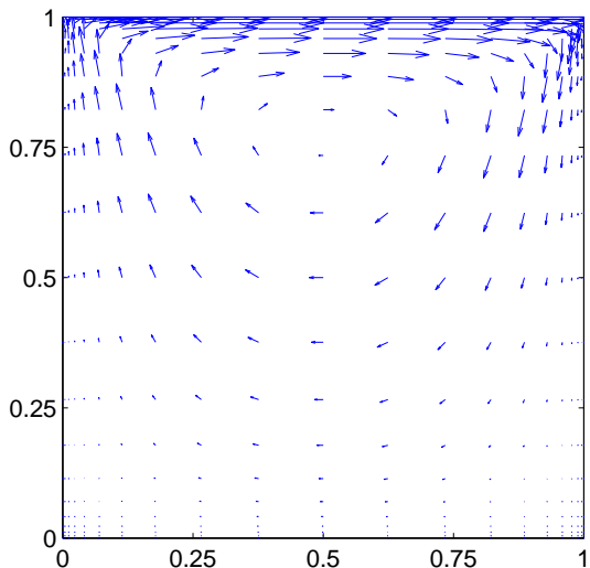
Figure 10: Velocity for non uniform mesh (Case B)
