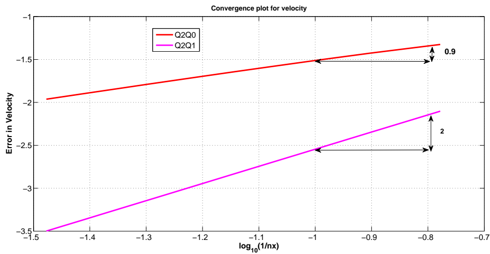
Figure 1: The error convergence of velocity
