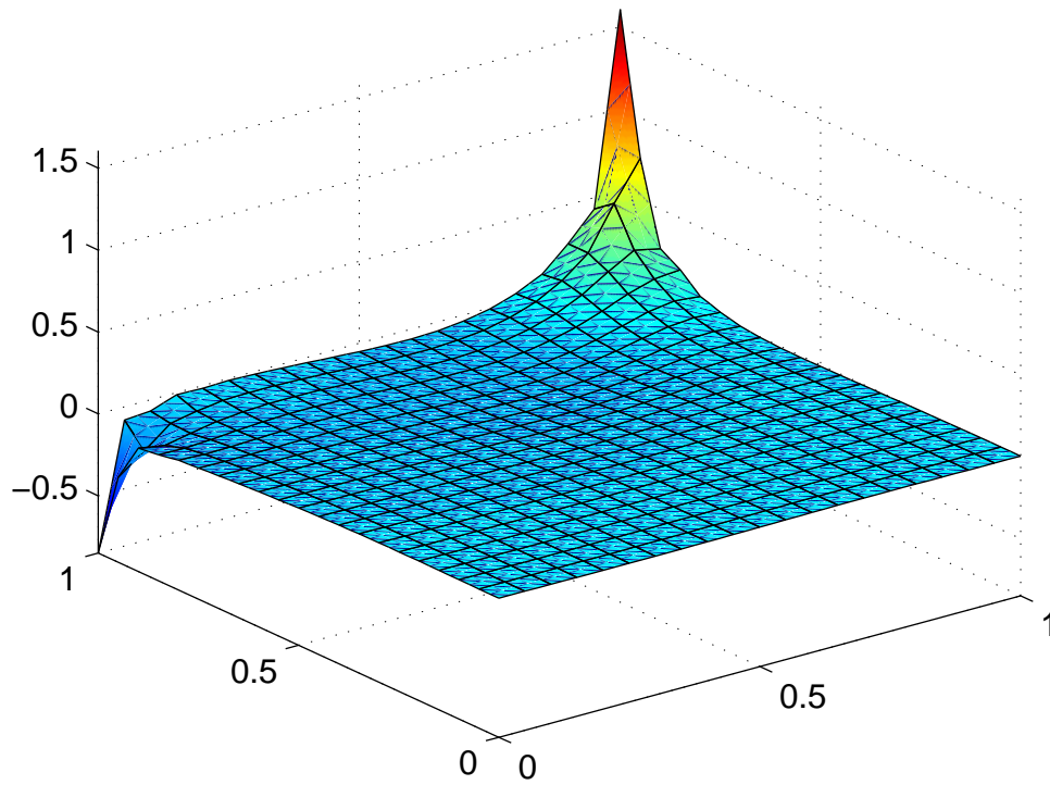
Figure 21: Pressure for Re 100
