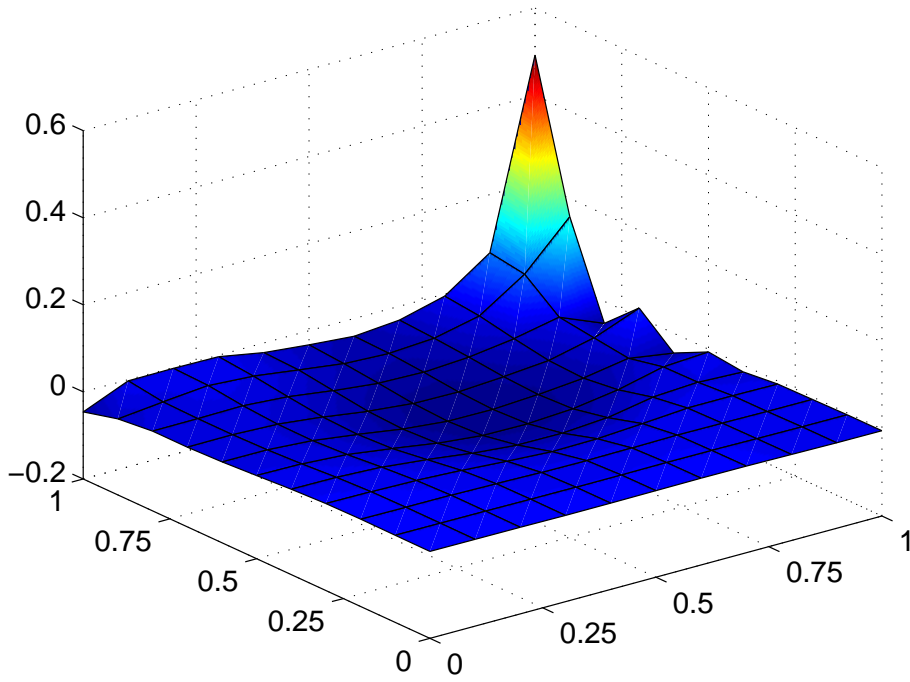
Figure 23: Pressure for Re 500
