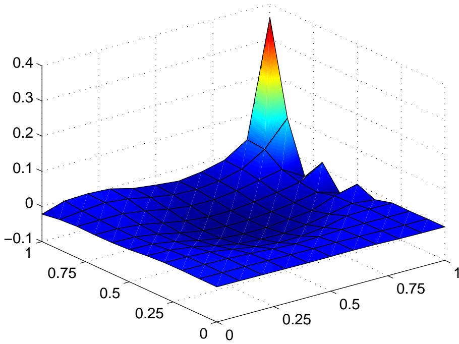
Figure 25: Pressure for Re 1000
