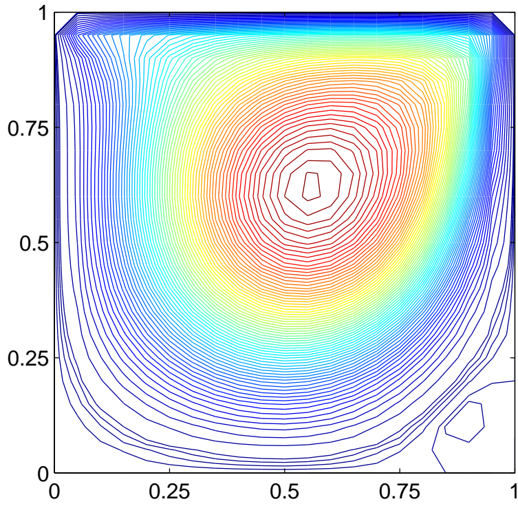
Figure 24: Streamlines for Re 500
