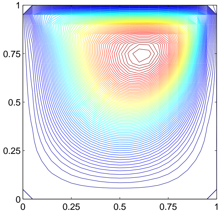
Figure 22: Streamlines for Re 100
