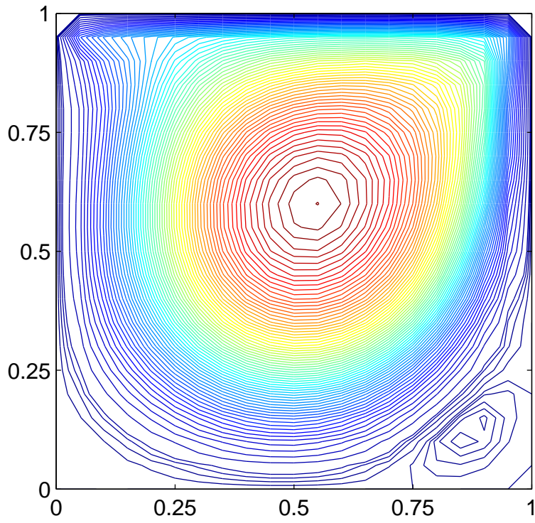
Figure 26: Streamlines for Re 1000
