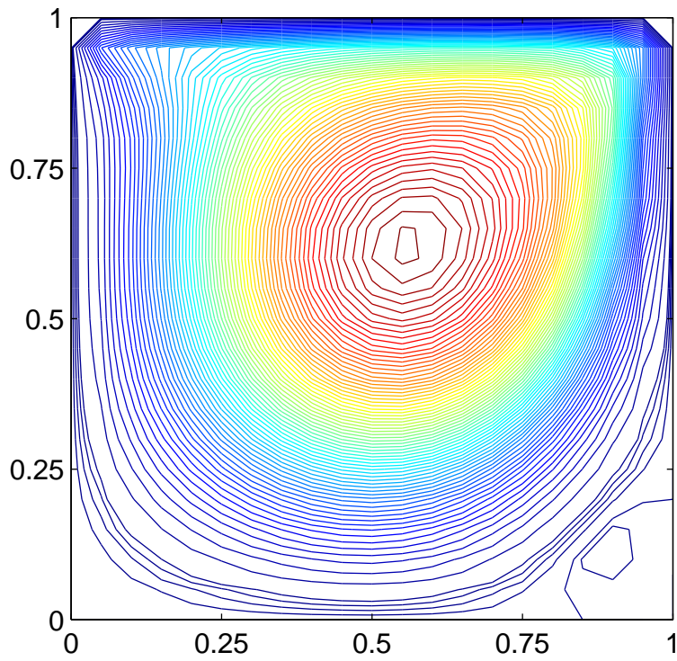
Figure 18: Streamlines for Re 500
