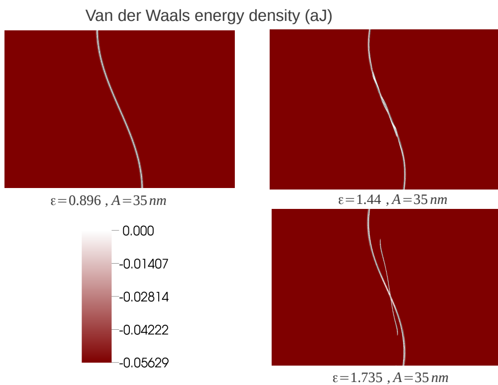
Figure 3.9: Van der Waals energy density along Graphene layer
