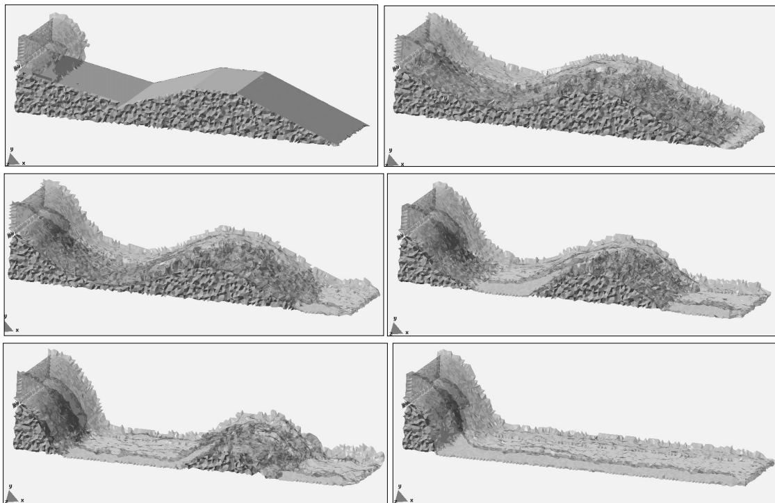
Figure 13: Erosion of a 3D earth dam due to an overflow streams.
